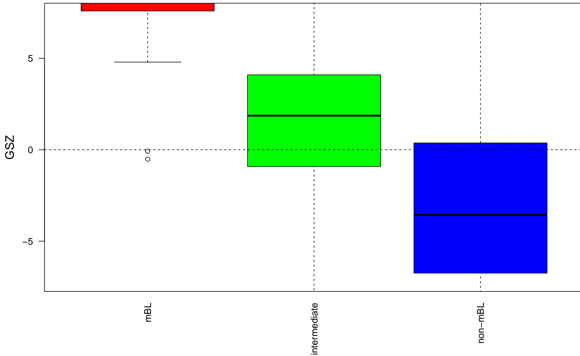
Pentrack_CRC_TCGA_group.over_C_normal_DN
